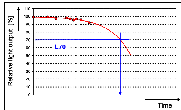
Figure 4: Degradation curve
